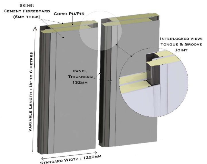
FastFix Double Wall
