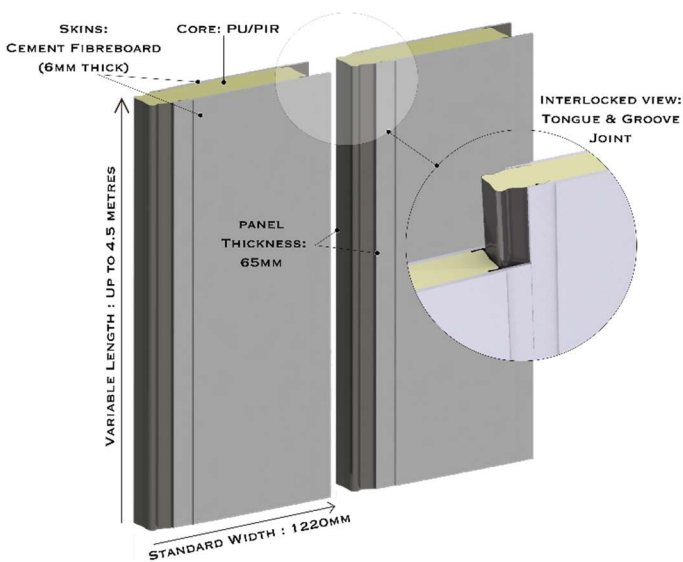
FastFix Single Wall
